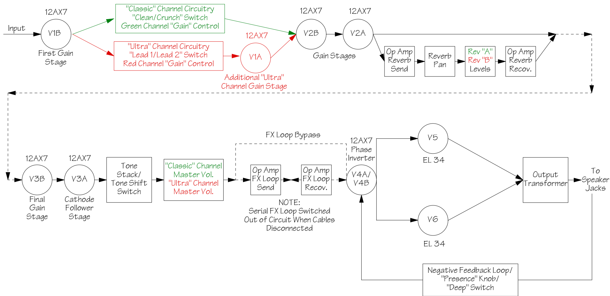
Marshall DSL 50 Signal Flow Diagram Drawn By: Lane Sparber 5/9/11
